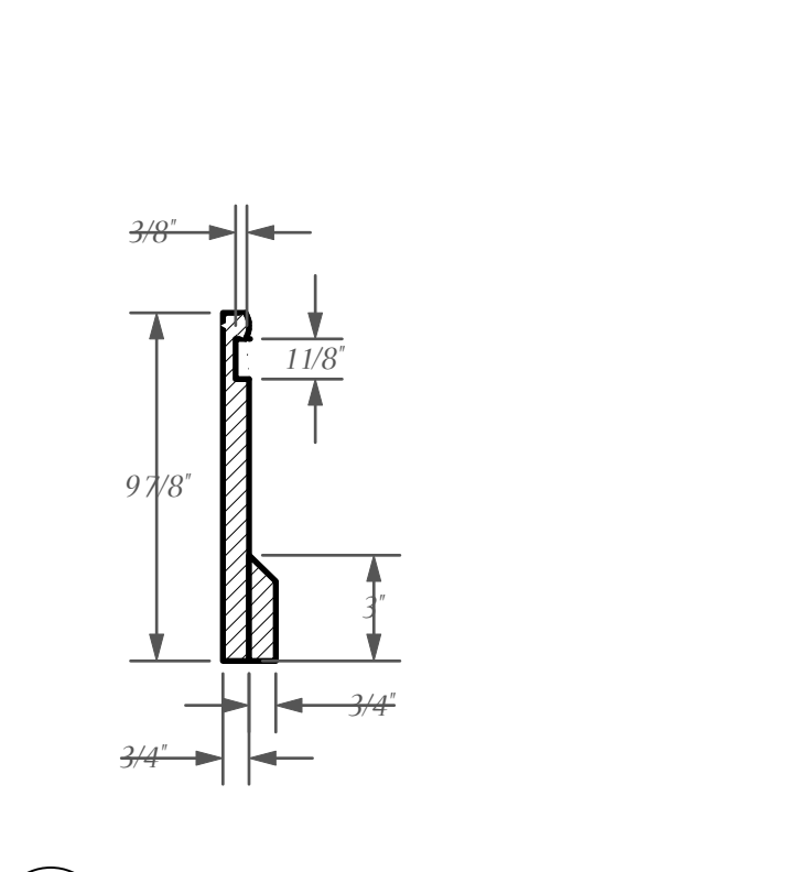
A DETAIL (A) 1ST FLOOR BASE Scale: 2"=1'-0"
