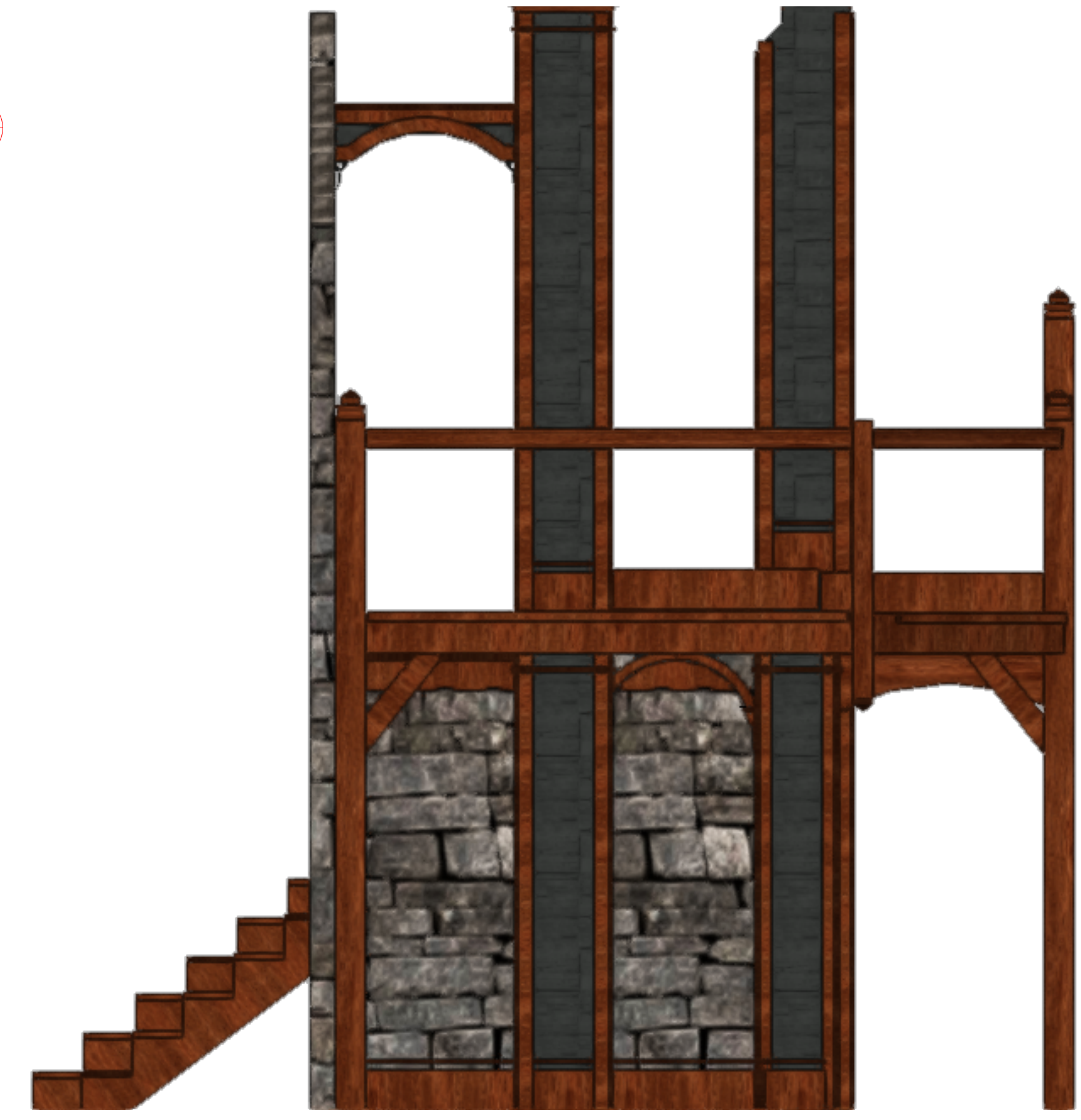
3 RENDERED FRONT VIEW Scale: 1/2"=1'-0"
