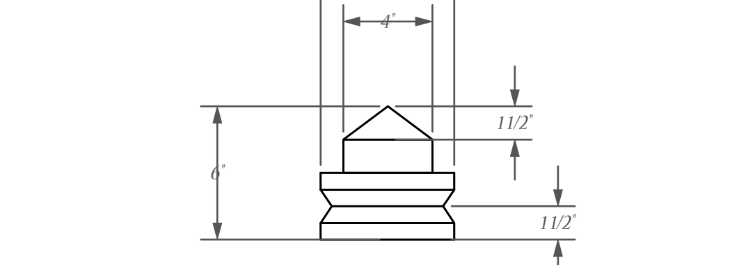
L DETAIL (L) POST TOP DETAIL Scale: 2"=1'-0"
