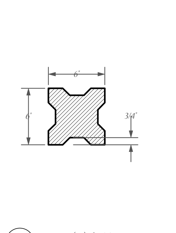
B DETAIL (B) 6 POST Scale: 2"=1'-0"
