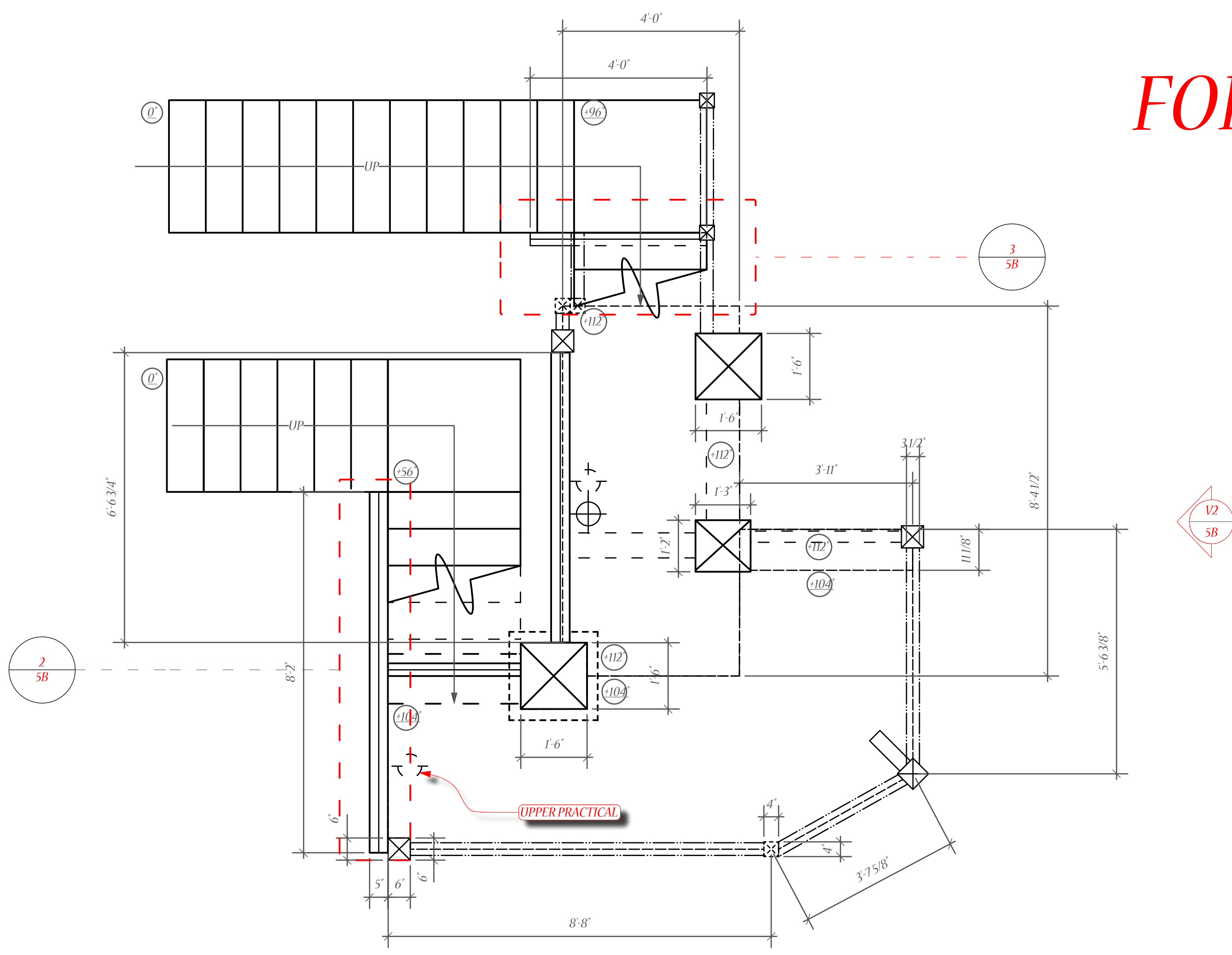
2 SR SEGMENT DETAIL VIEW SCALE: 1/2"=1'-0"
